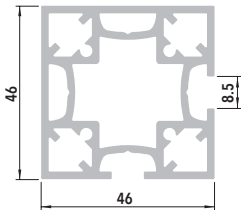
REF. S 47
