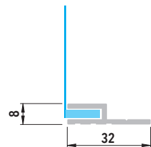
REF. T3CN
