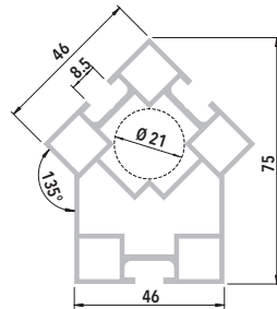
REF. PX 4345
