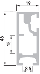
REF. PH 1452
