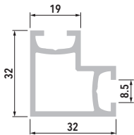
REF. GS 220
